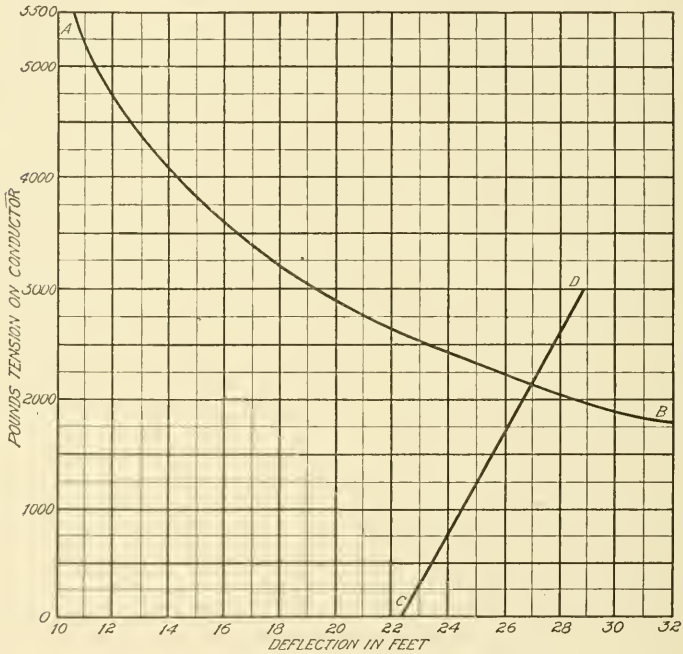
Fig. 44. Graphical Solution of Example, Page 71
